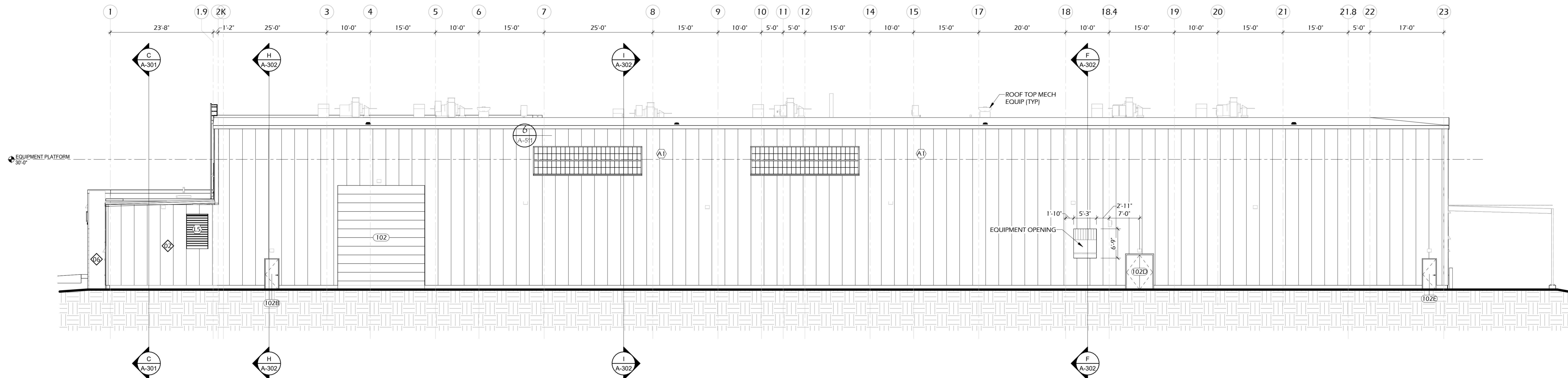
2 NORTH SCALE: 3/32" = 1'-0"
